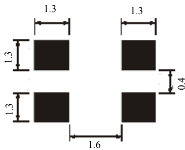
Pad layout
